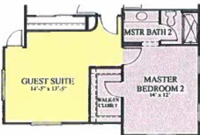
#4 OPTIONAL GUEST SUITE & OPT. MSTR BEDRM 2 REPLACES BEDROOM #3 & GARAGE
